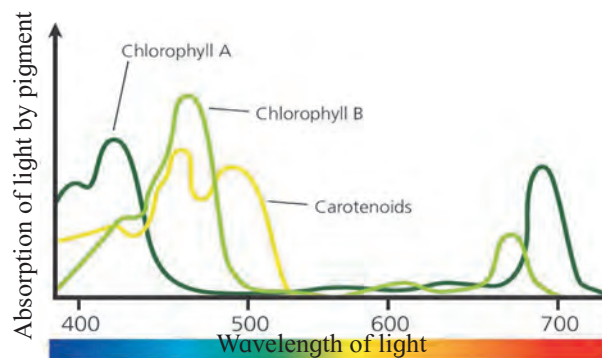
Graph 12.3 Absorption spectrum
